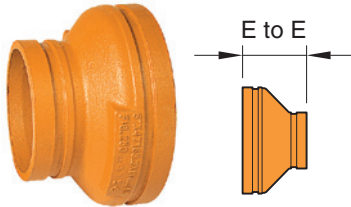
Figure 250 Concentric Reducer Cast
