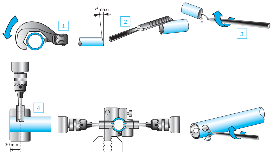
Drilling jig for aluminium pipe ref. 6698 01 02
