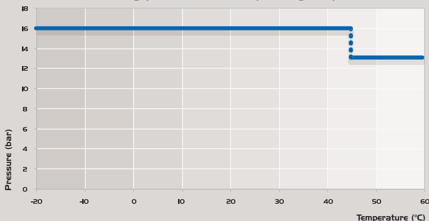
Maximum working pressure versus operating temperature
