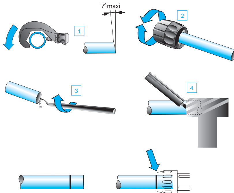
Pipe cutter for aluminium pipe ref. 6698 03 01
