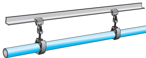
Push-on type beam clamps
