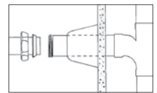
Slip joint thread for copper DWV pipe.
