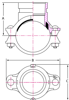
Fig. 65MG & 66MG Mechanical Tee, Grooved
